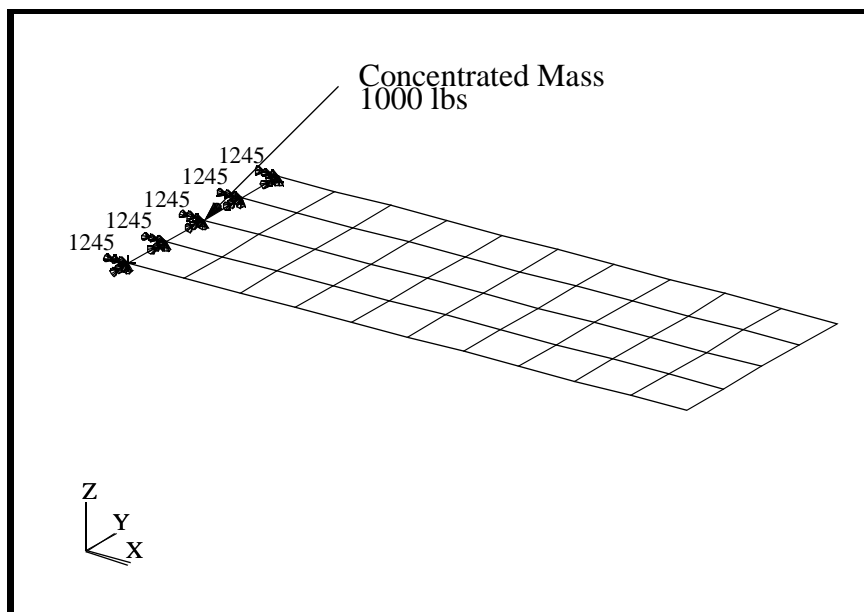
Figure 7.1 - Loads and Boundary Conditions
